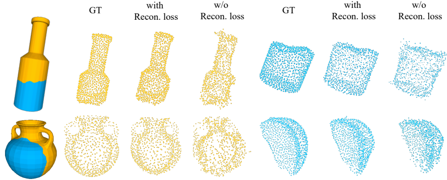
Fig. 8. Ablation study on complementary shape prediction.
