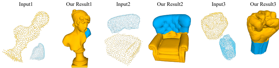
Fig. 7. Additional unseen examples.
