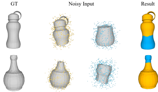
Fig. 6. Qualitative examples of reassembling noisy point clouds.
