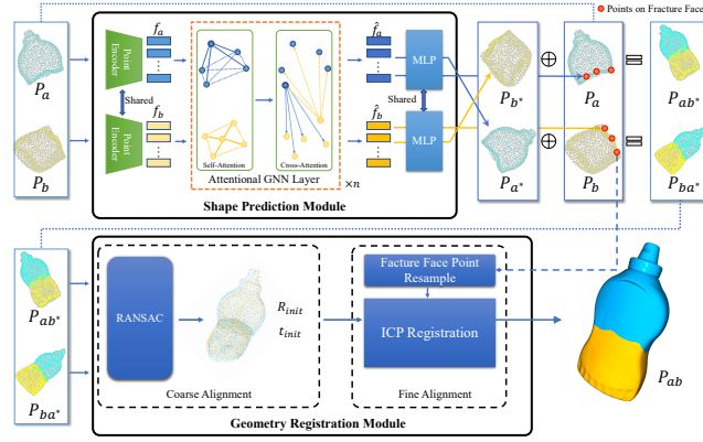
Fig. 1. Pipeline. Our method mainly contains two components: a shape prediction module and a geometric registration module. The former consists of a point cloud encoder based on DGCNN, a graph network with a specifically designed attention mechanism, and an output layer based on MLP. Given two input fragments P_a and P_b , it learns to predict both the fracture face points and their complementary shapes P_{b^*} and P_{a^*} , resulting in combined shapes P_{ab^*} and P_{ba^*} , respectively. The geometric registration module takes P_{ab^*} and P_{ba^*} as input and employs RANSAC to achieve an coarse alignment \{R_{init}, t_{init}\} between P_a and P_b , followed by ICP acting on the predicted fracture face points to compute a refined alignment for the final reassembly P_{ab} .
