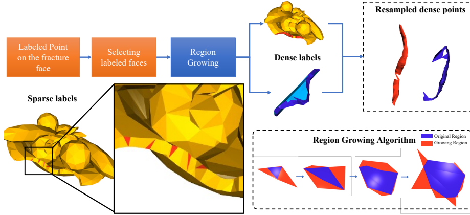
Fig. 2. Dense points are sampled based on the predicted fracture surface points and their associated mesh faces. Region growing is applied to fill the gaps between mesh faces and enable dense sampling.
